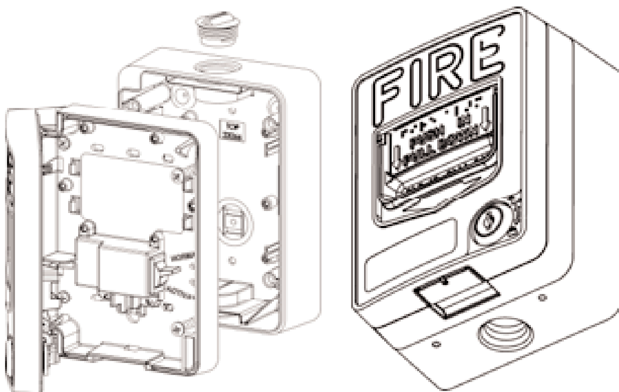
SB-I/O shown assembled to Pull Station (Pull Station Sold Separately)
