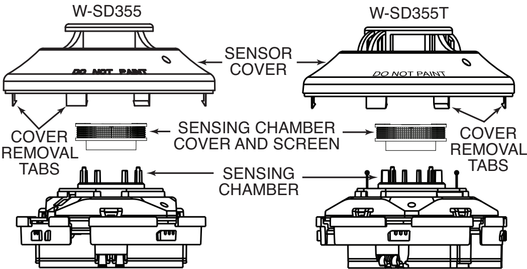
FIGURE 5. DETECTOR COMPONENTS:
